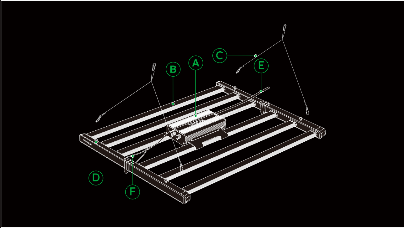
A.LED Drivers B.LED Bars C.Lance Hanger D.Ring Screw E.Input Power Cord F.Interconnect Cable
